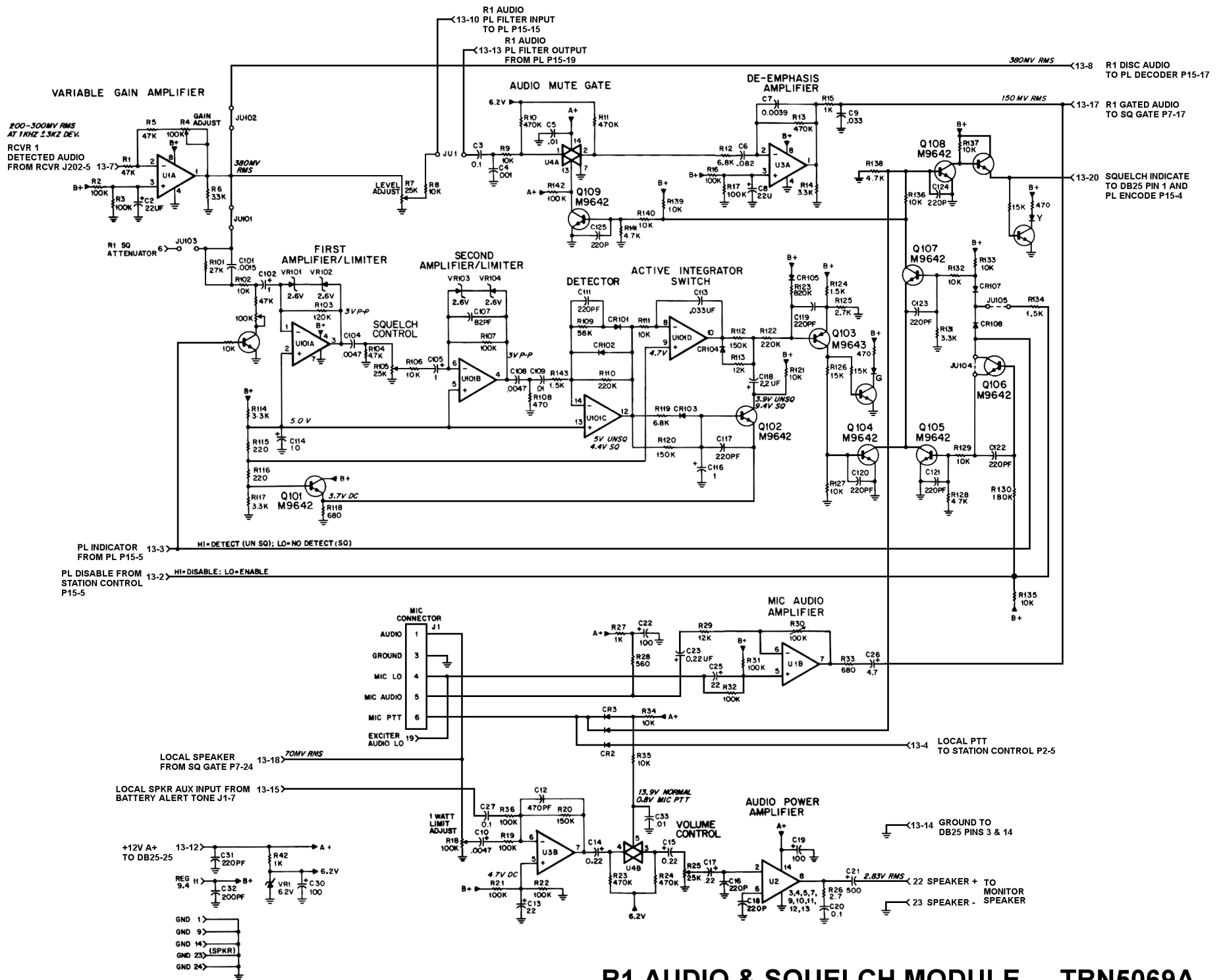
R1 AUDIO & SQUELCH MODULE - TRN5069A
