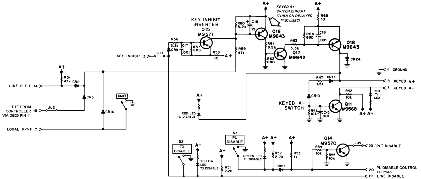
Station Control Module - TRN5321A
